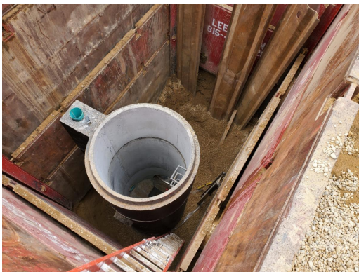
Manhole construction
