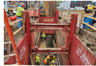
Sanitary casing
