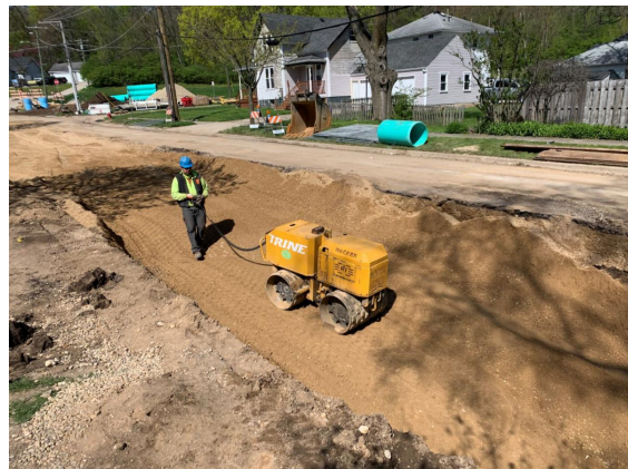
Compaction of the trench backfill
